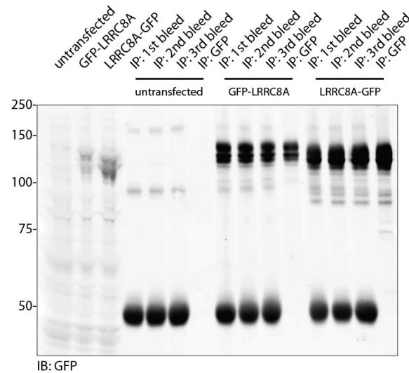
IB: GFP
